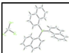
Fig. 1. The molecular structure of the title compound with 50% probability ellipsoids for non-H atoms.
